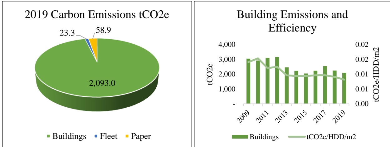
Figure 1: 2019 Carbon emissions by source.
